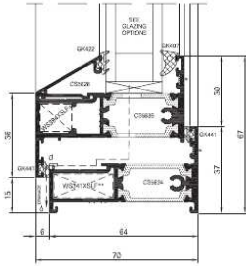
General arrangement showing the outer frame, open out sill detail, externally beaded vent.
