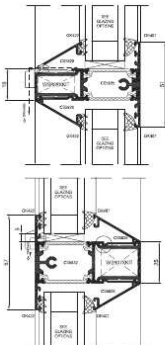
General arrangement showing mullion/transom details, externally/ internally beaded section.
