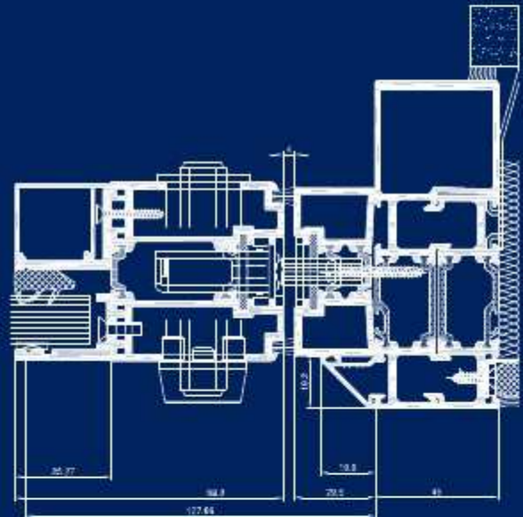
General Arrangement showing Comar 7Pi CD with the Security Jamb Locking Detail
