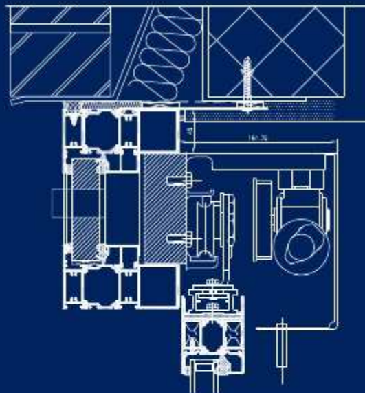
General Arrangement showing Comar 7Pi CD Automatic Door Head Detail
